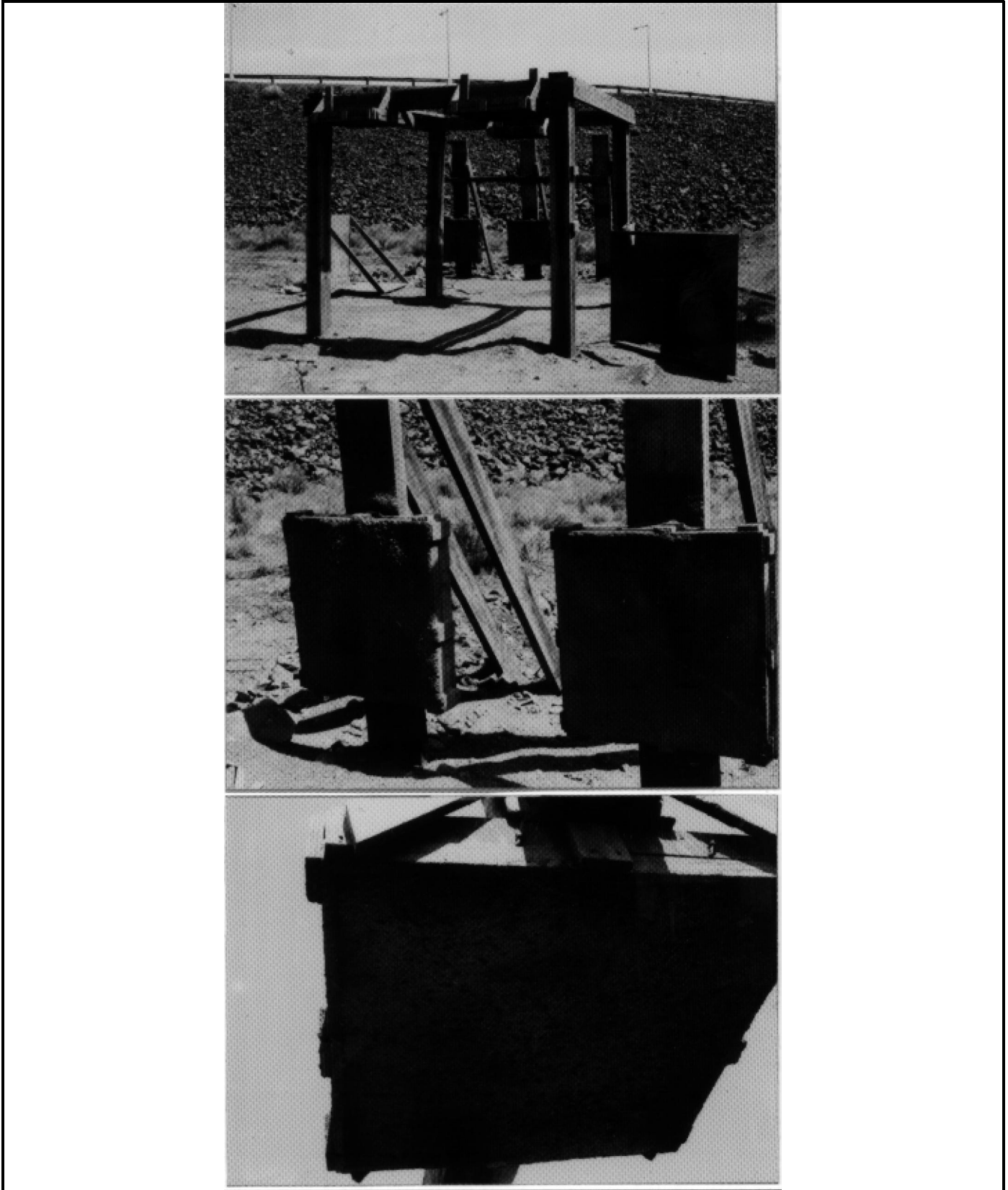
Figure 5-2. Test panel frame system
