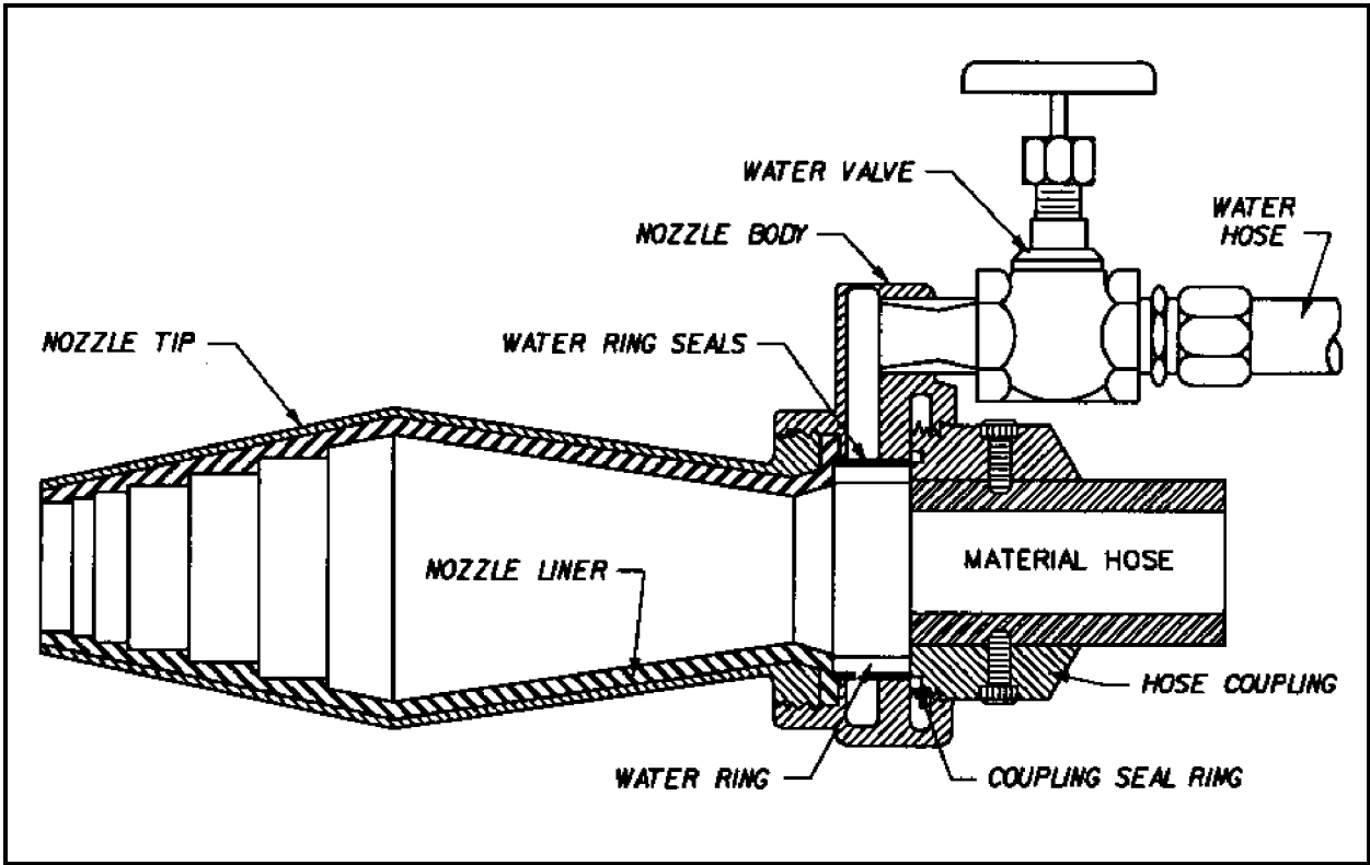
Figure 4-8. Typical dry-mix nozzle (paragraph A-2, ACI 1991c; copyright permission granted by ACI)
